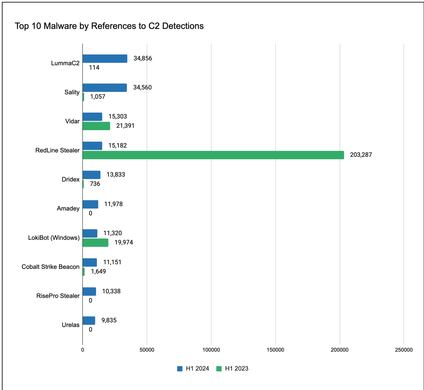
Figure 2: The top ten malware families by number of references to C2 detections in H1 2024 and H1 2023 (Source: Recorded Future)
