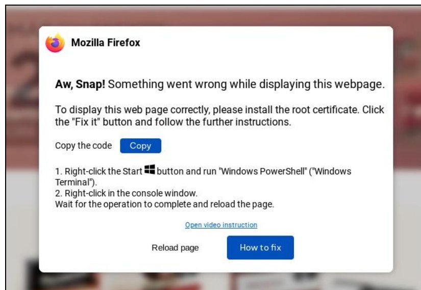
Figure 3: Phishing message in ClearFake's campaign prompting victims to copy malicious PowerShell code (Source: ReliaQuest )
