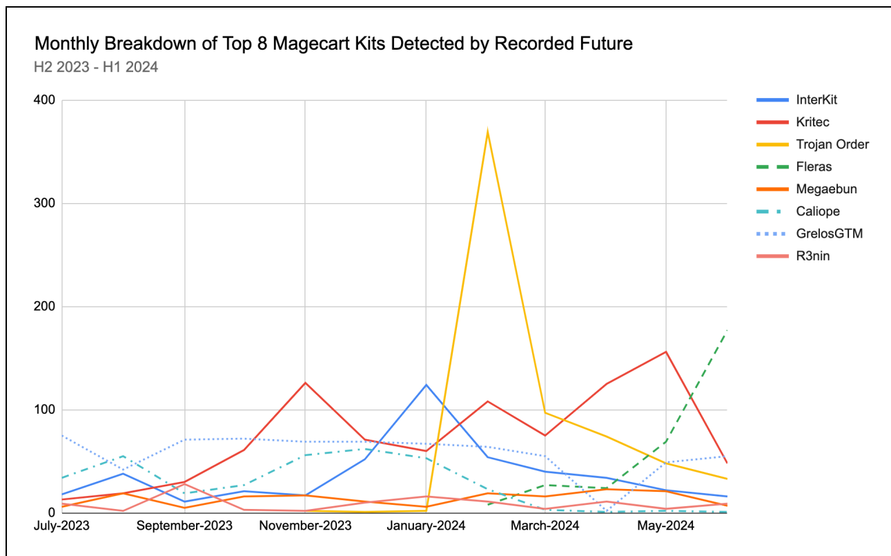
Figure 6: Intrusions associated with the top eight Magecart kits Recorded Future detected between H2 2023 and H1 2024 (Source: Recorded Future)
