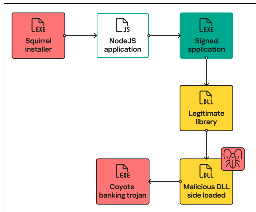
Figure 4: Overview of Coyote's infection chain (Source: Kaspersky )
