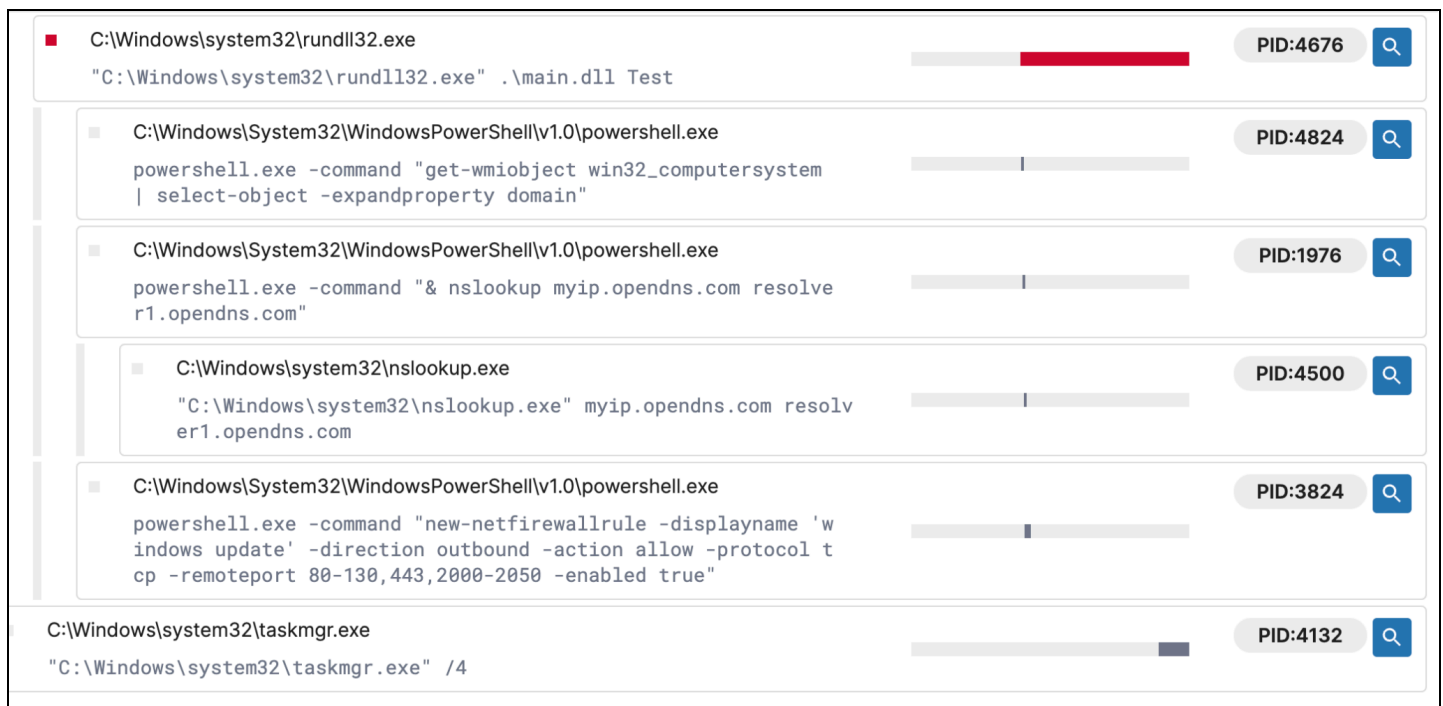
Figure 10: PortStarter commands (Source: Recorded Future Malware Intelligence )
