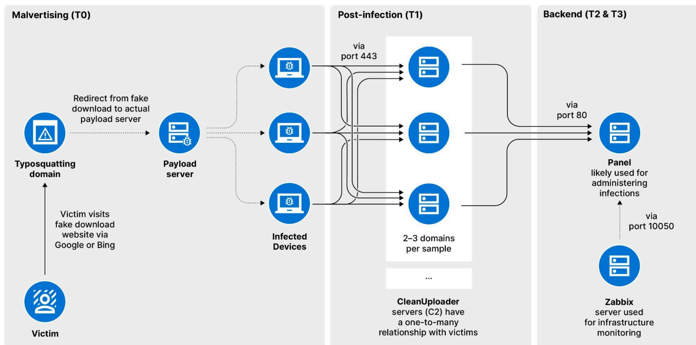
Figure 12: Rhysida multi-tiered infrastructure used for CleanUpLoader-based intrusions (Source: Recorded Future)
