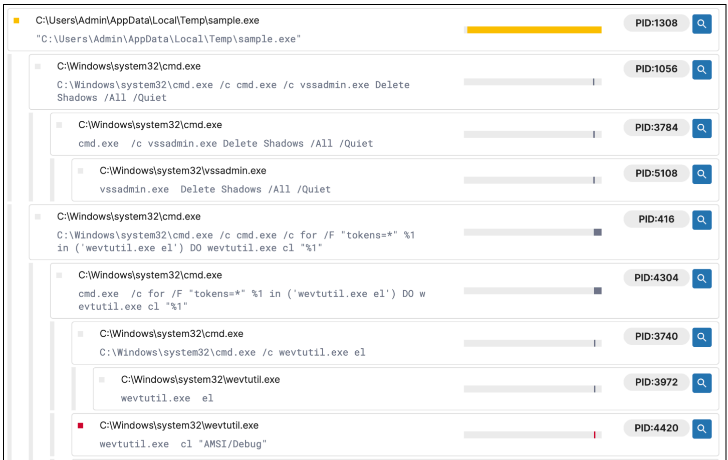
Figure 6: Rhysida ransomware command lines to delete shadow copies and Windows event logs (Source: Recorded Future Malware Intelligence )
