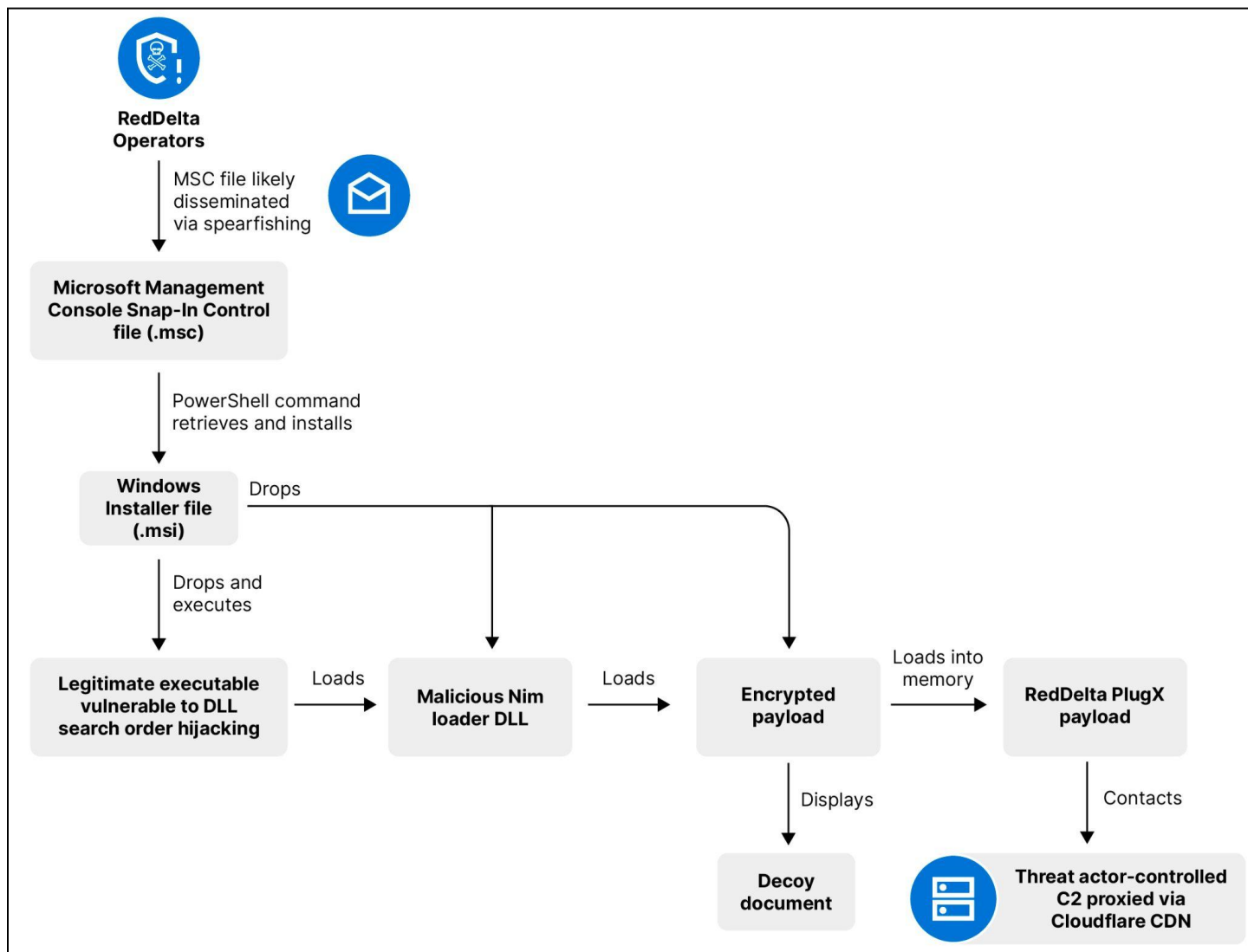
Figure 8: Updated RedDelta infection chain observed in May 2024 (Source: Recorded Future)
