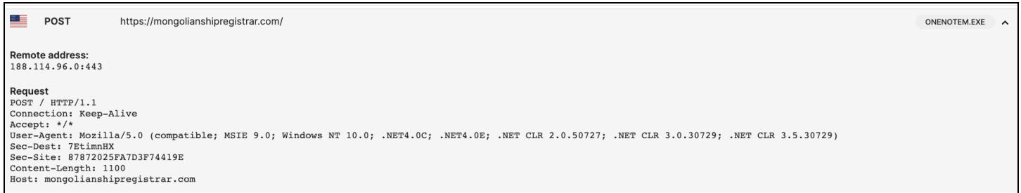
Figure 4: RedDelta PlugX C2 headers observed in highlighted sample (Source: Recorded Future Malware Intelligence)
